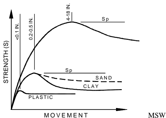
FIGURE 8 - LARGE STRAIN BEHAVIORS
