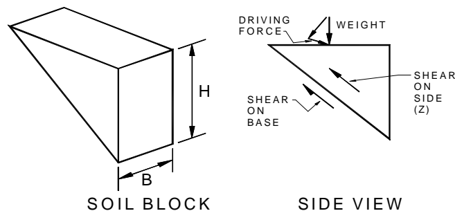
FIGURE 3 - SIMPLIFIED 3D MODEL
