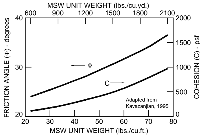
FIGURE 11 - MSW STRENGTH PARAMETERS vs DENSITY
