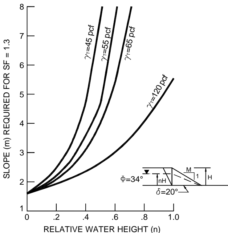
FIGURE 15 - SLUDGE LANDFILL STABILITY
