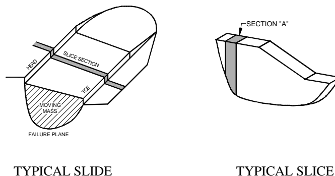
FIGURE 4 - FAILURE BLOCKS
