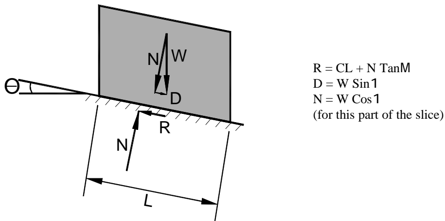
FIGURE 5 - FORCE RESOLUTION
