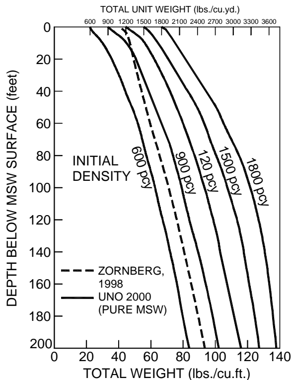
FIGURE 10 - MSW DENSITY vs DEPTH
